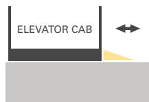
Slab with RAM's No Pit (small ramp required for 3in rise)
